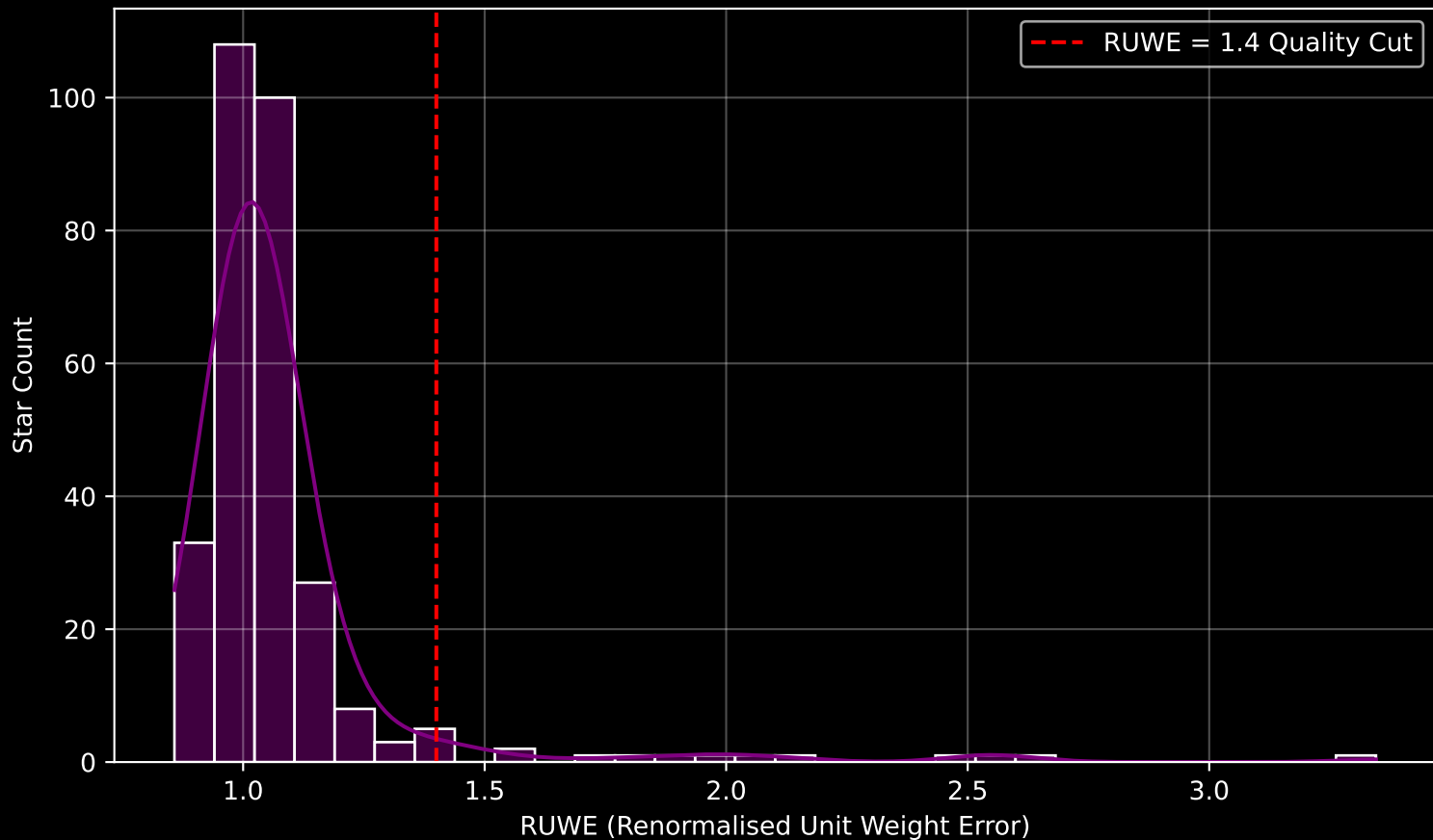
GAPOGEE DR17 Field [169+12] RUWE Distribution (n= 296)
