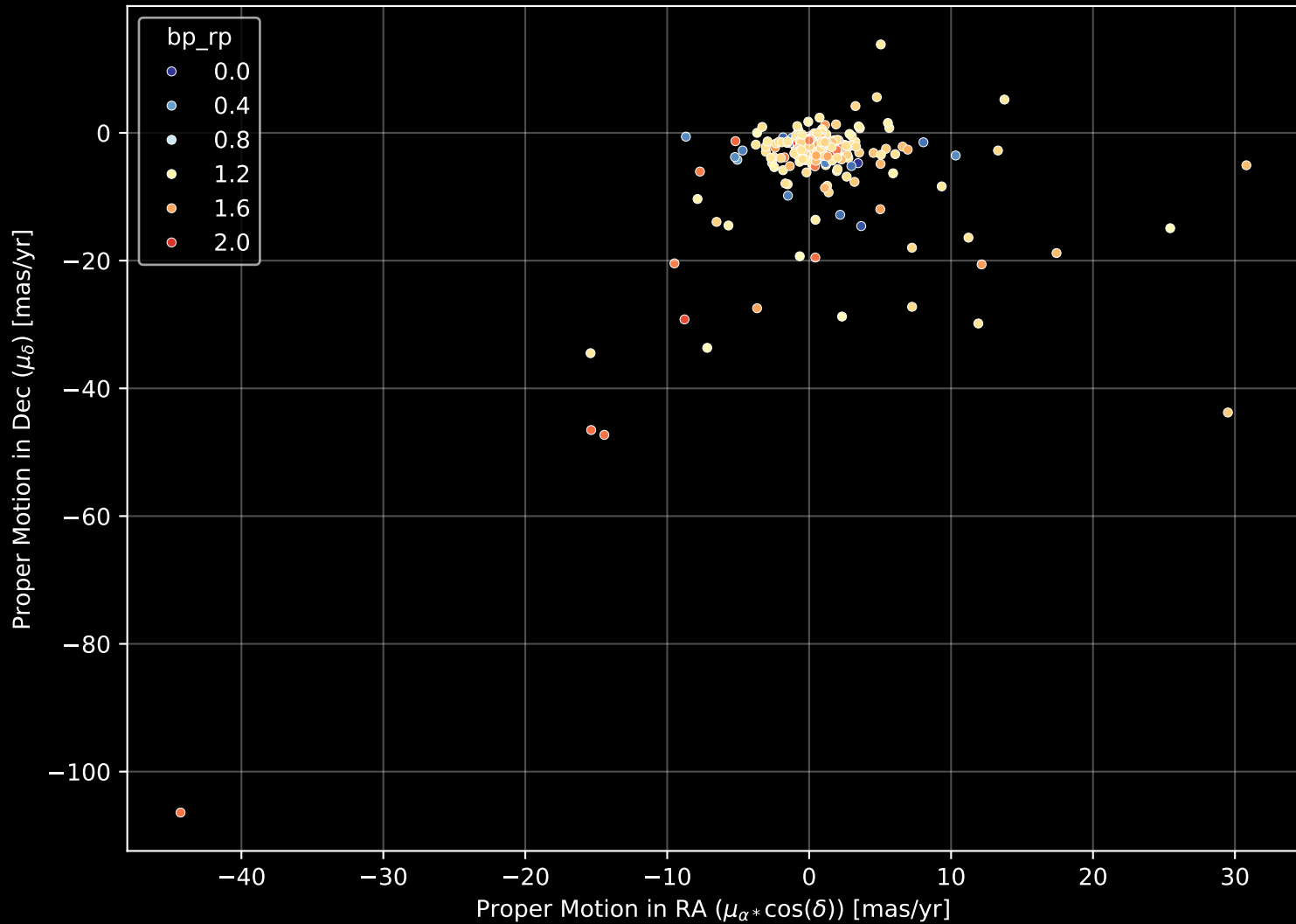
APOGEE DR17 Field: [169+12] Proper Motion Diagram (n= 299)
