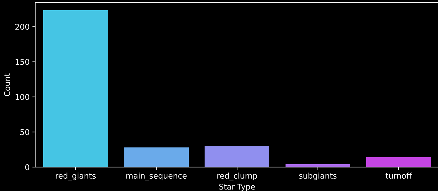
APOGEE DR17 Field: [169+12] Count plot of Star Type
