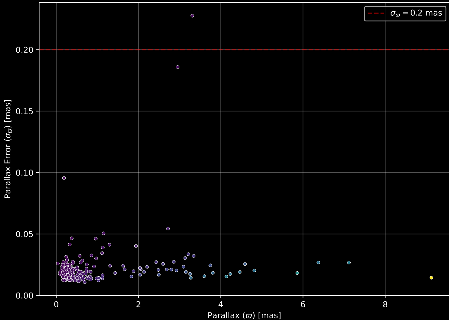
APOGEE DR17 Field: [169+12] Parallax Quality (n= 299)
