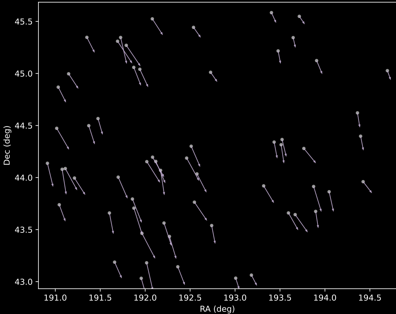
APOGEE DR17 Cluster 9 Proper Motion Vectors (n=60)
