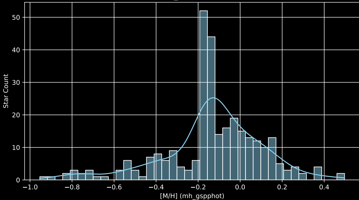
APOGEE DR17 Field: [169+12 [M/H] (mh_gspphot) (n= 298)
